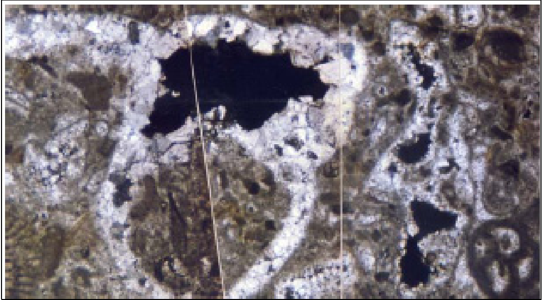
Figure 4. Mouldic porosity and blocky spar cementation on gastropode. Photo base is about 7 mm long.
