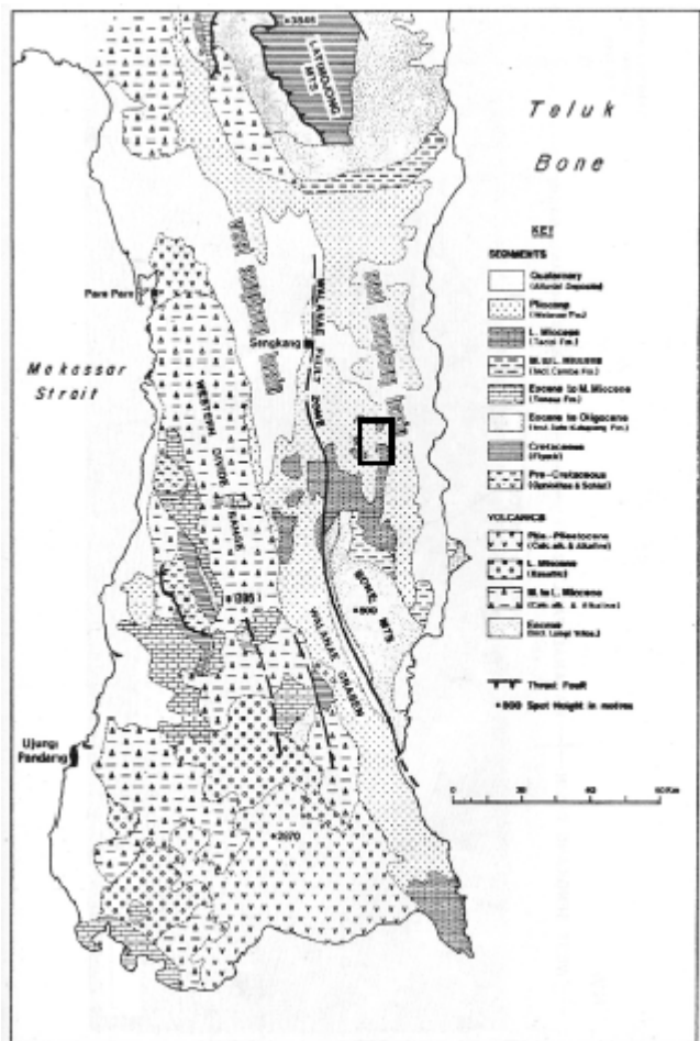
Figure 1. Regional geology of southern arm Celebes (Sukamto, 1982). Research area is shown by open square and located in the East Sengkang Basin.
