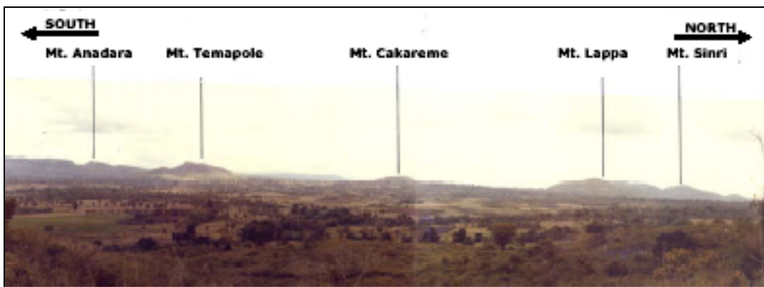
Fig. 2: Ridges and pinnacles morphology of the western part Tacipi carbonate field. On the foreground is relatively flat inter-reef area. Photograph from the eastern ridges.
