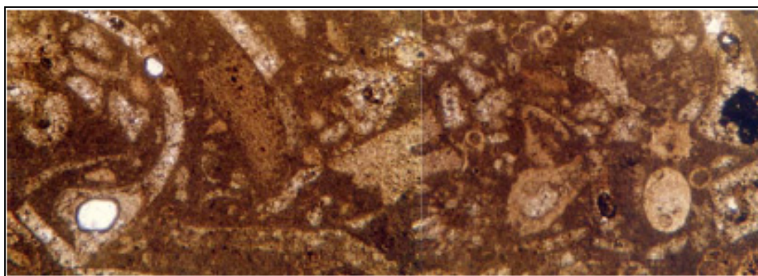
Figure 6. Rudstone sample under microscope showing various reef materials as bioclastic fragments which are enclosed by wackestone groundmass. Photobase is about 10 mm long.
