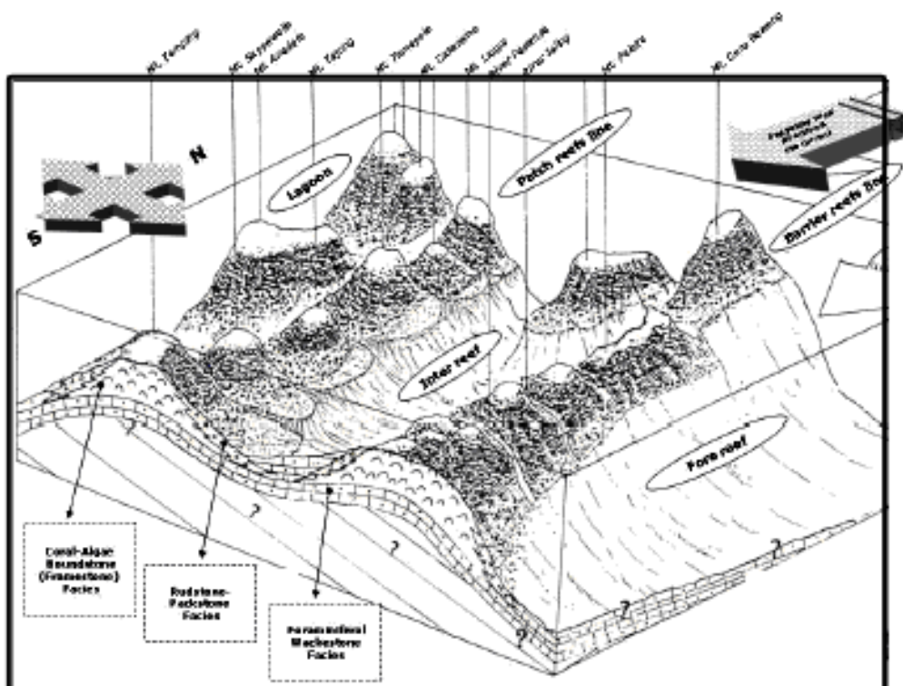
Figure 8. Hypothetical block diagram showing paleo-environment of reef complex of Tacipi area. Talus or reef debris distributed more extensive in the southern part due north-south wind trend and sea current. Patch reefs are distributed between Temapole and Tamping, whereas barrier reefs between Curu Baweng and Pasampa river.
