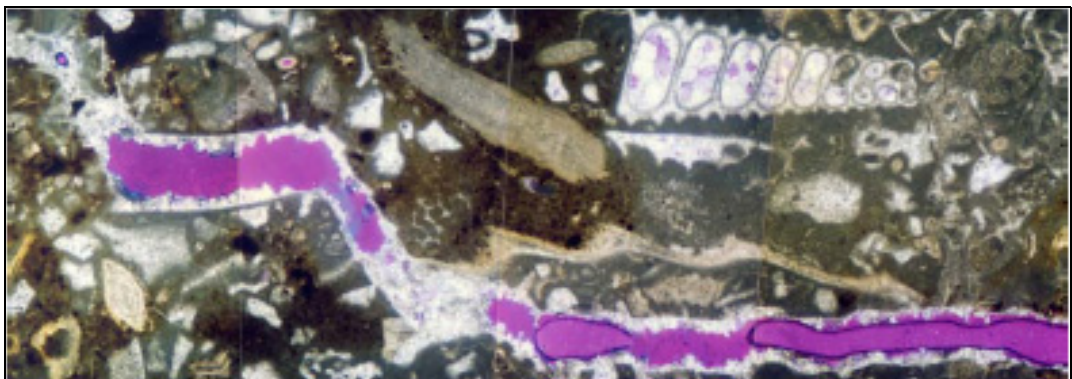
Figure 7. Vuggy and mouldic porosity which partly blocked by sparry calcite. Photographed in cross polar position with gypsum comparator. Photo base is about 10 mm
