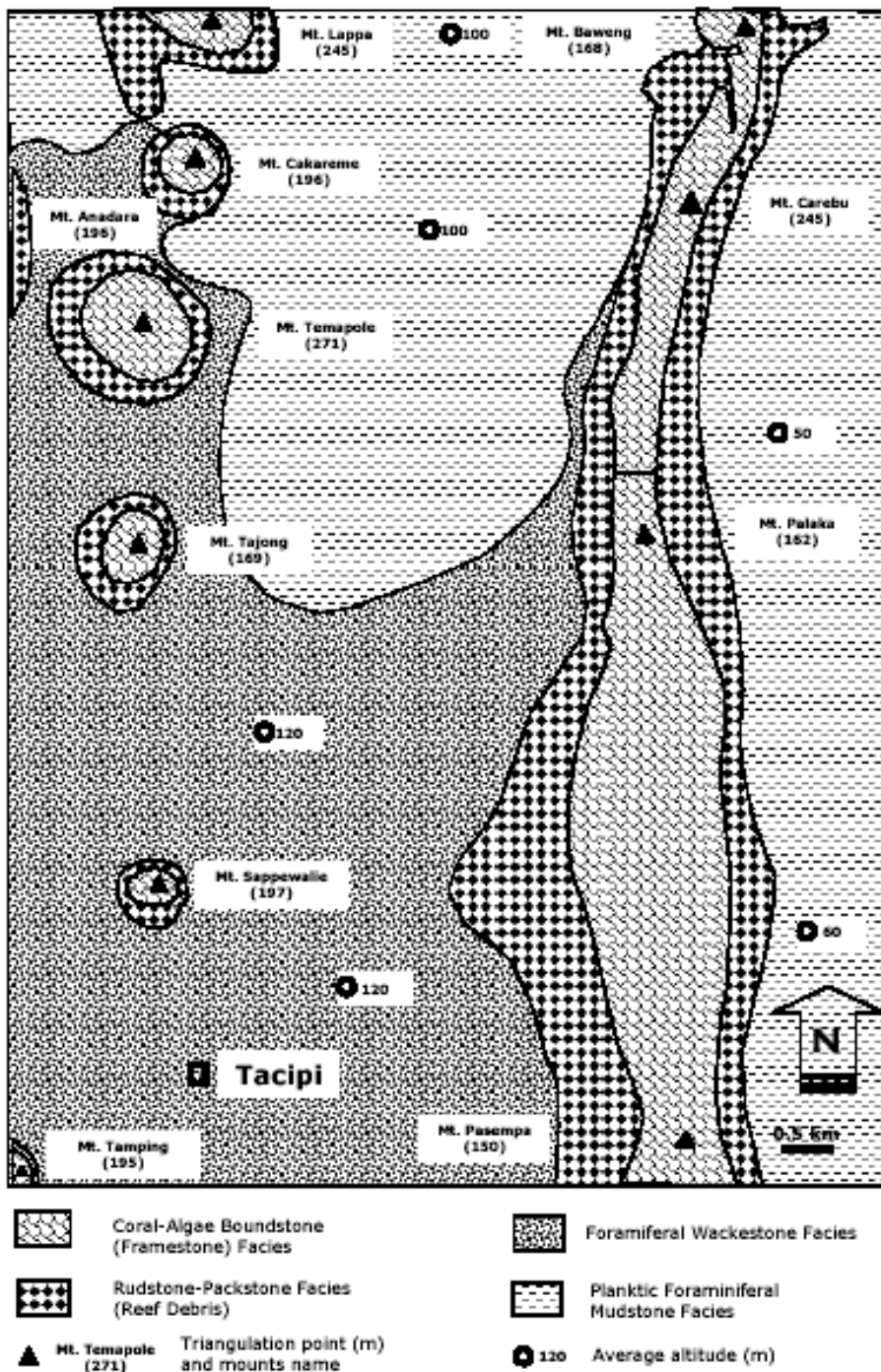
Figure 3. Simplified carbonate facies map of Tacipi area.
