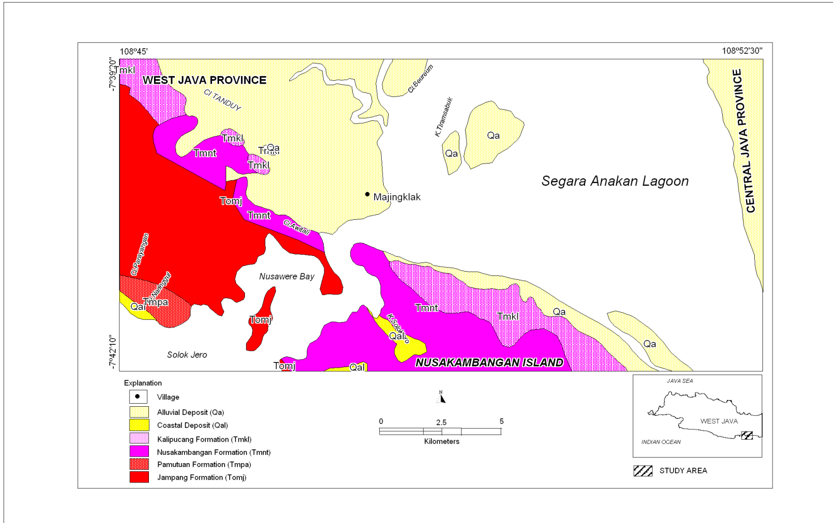
Figure 1. Geological map of Sagara Anakan and adjacent area
