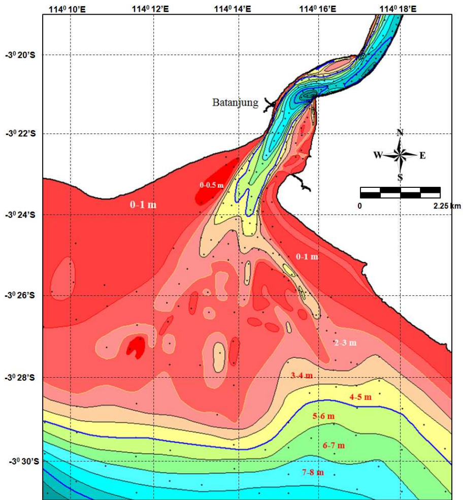
Figure 2. Bathymetry around the River Mouth of the Kapuas Muring River, (Priohandono, et. al, 2010)
