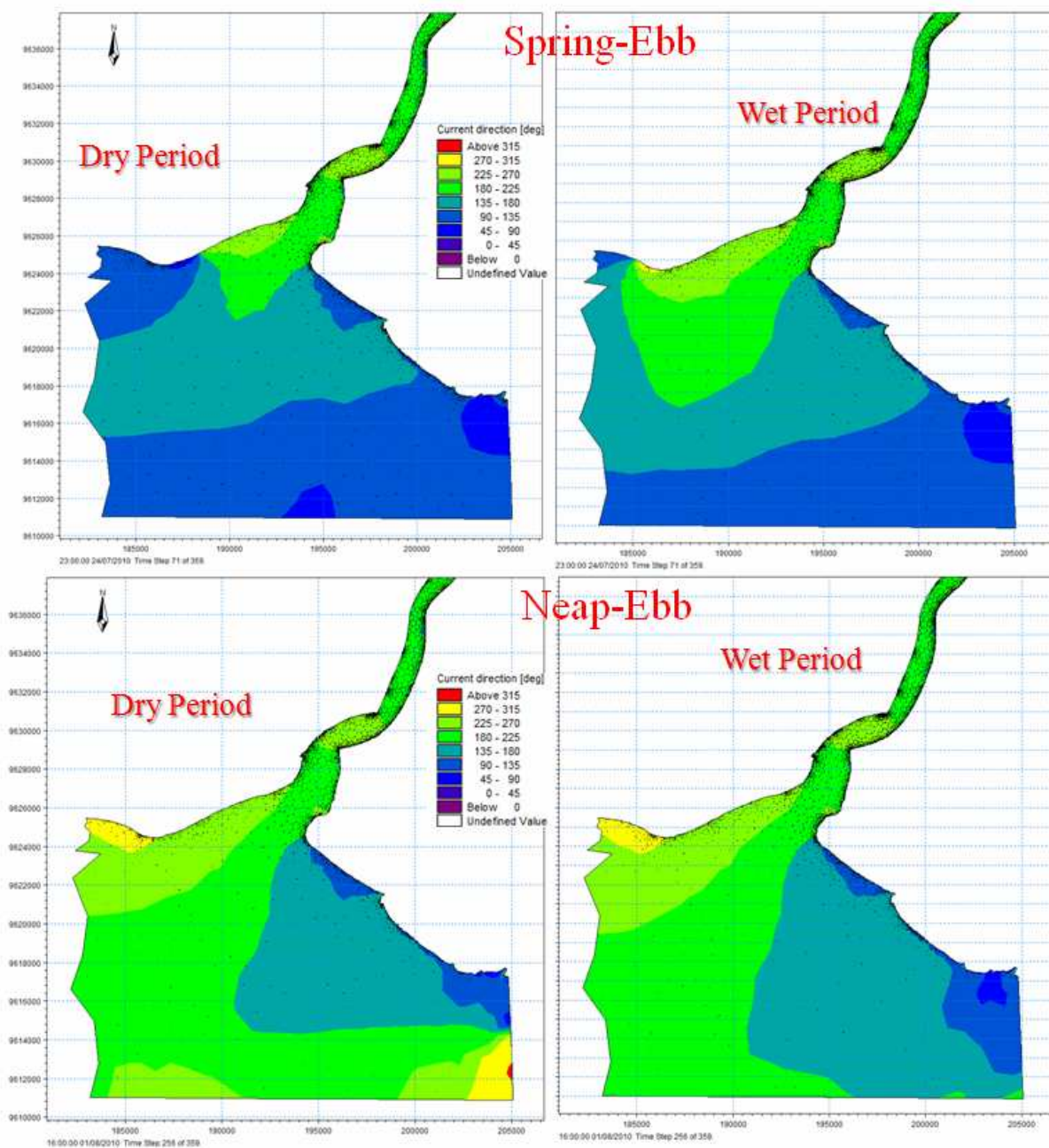
Figure 15. Current Direction (Ebb Condition)
