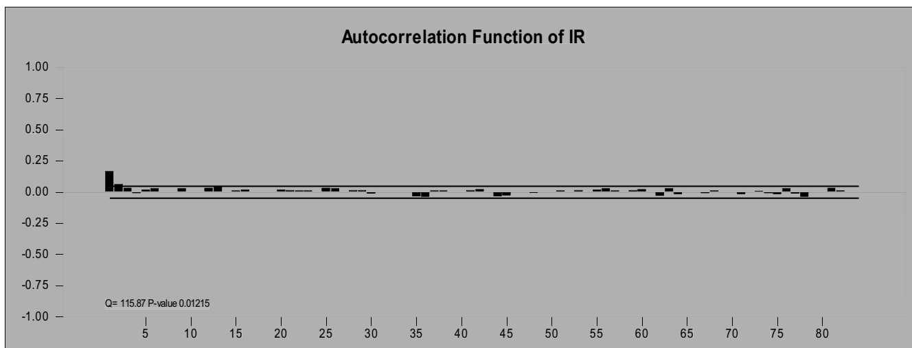
Figure 2. Autocorrelation Function for Insurance Sector Stock Returns in Nigeria 02 January 2009 to 02 February 2016
