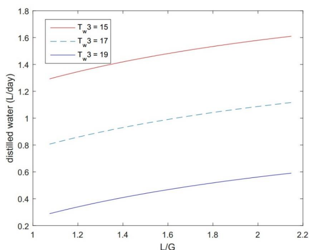
Fig. 4 Optimum production changes due to changes in the ratio of input water to input air
