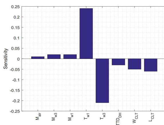
Fig. 3 Sensitivity analysis of humidification and dehumidification parameters
