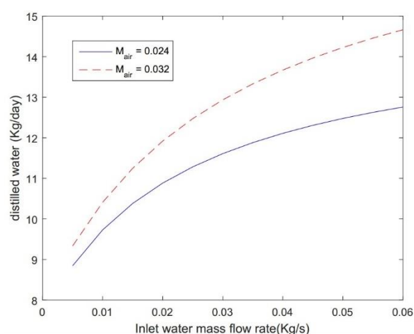
Fig. 2a Distilled water changes to inlet water flow rate
