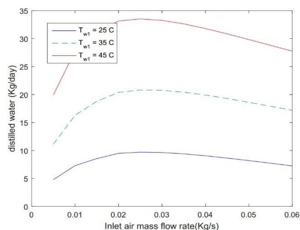
Fig. 2b Distilled water changes to inlet air flow rate
