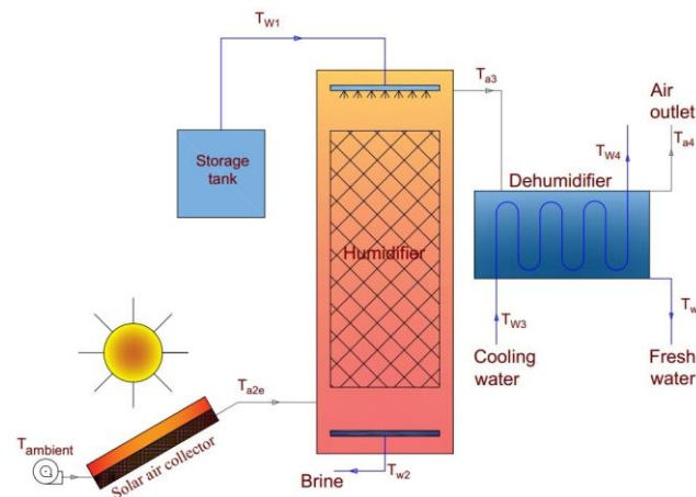
Fig. 1 The proposed model schematic
