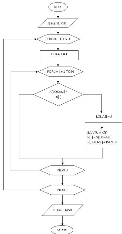
Gambar 1. Flowchart metode Straight Selection
