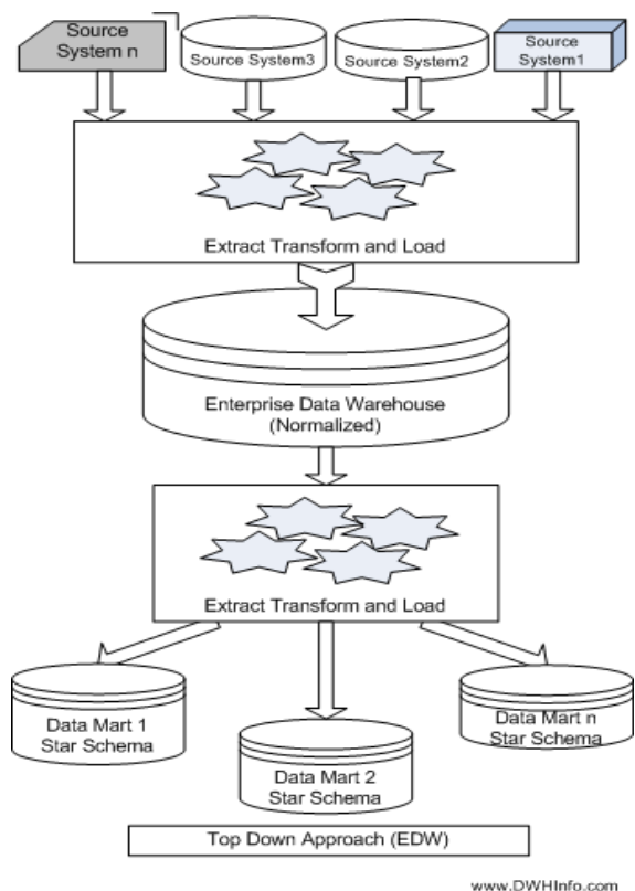
Gambar 2. Pendekatan Top-Down .
