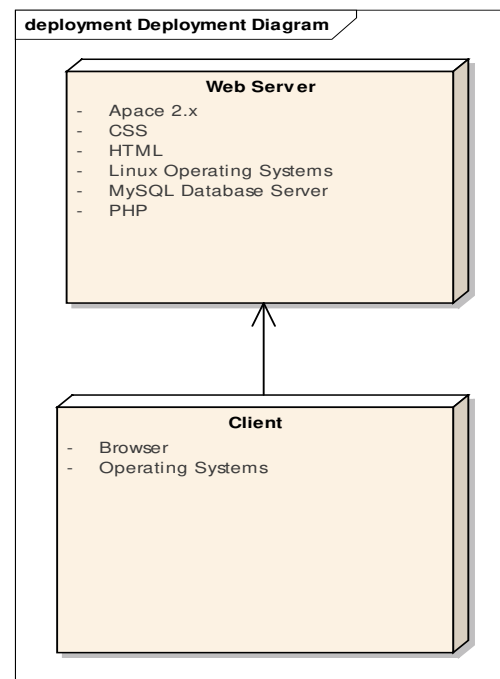
Gambar 6. Deployment Diagram
