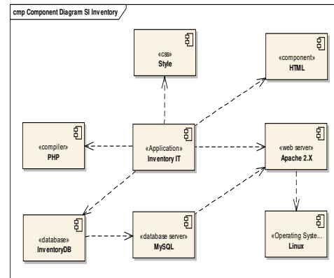
Gambar 5. Component Diagram SI Inventory
