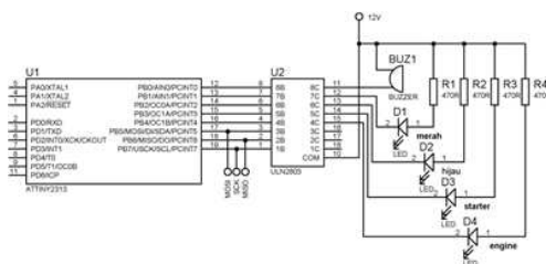
Gambar 8. Rangkaian buzzer
