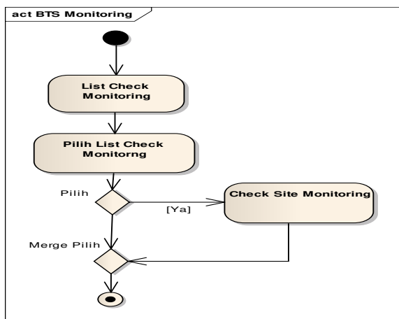
Sumber: Subhan & Mulyani (2015) Gambar 3. Activity diagram menu monitoring
