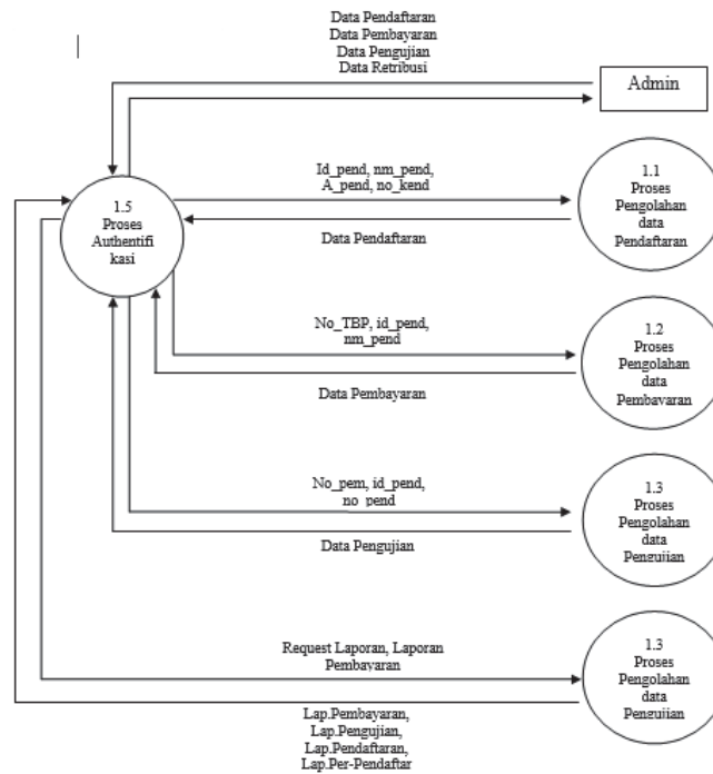
Gambar 3. DFD Level 1
