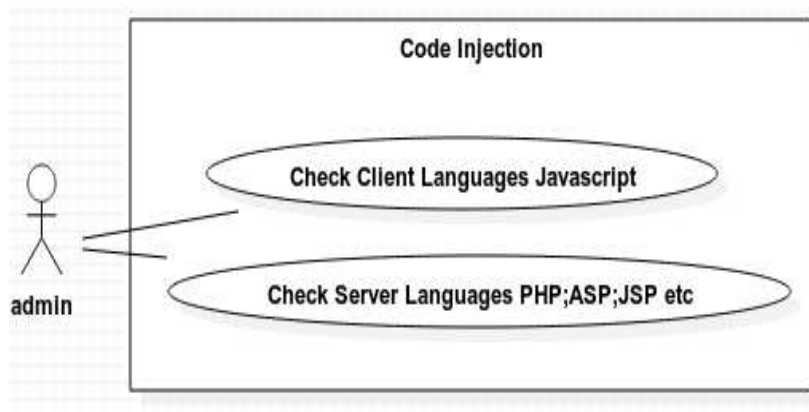
Gambar 6. use case diagram : code injection
