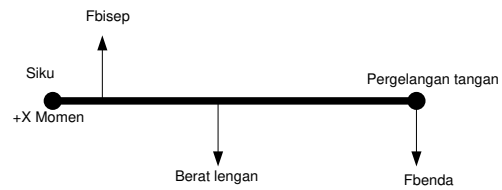
Gambar 1 Diagram benda bebas model tangan-siku. (Iridiastadi & Yassierli, 2014)
