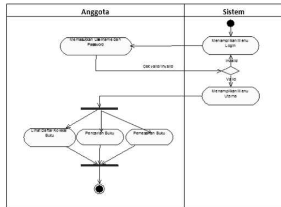
Gambar 3. Activity Diagram
