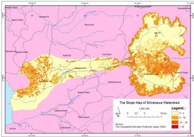
Figure 3. Slope map
