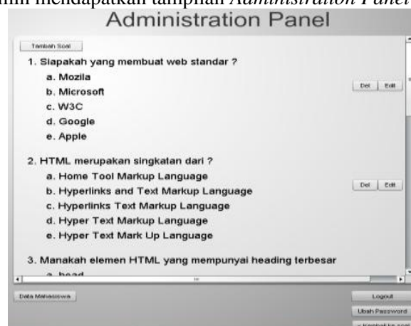
Gambar. 13. Administration Panel
