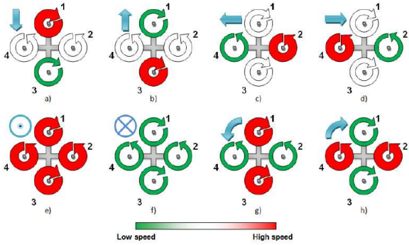
Fig. 2 Manauver of quadcoptere
