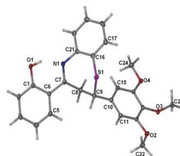
Fig. 2 Xray crystal structure
