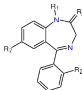
Fig. 1 Molecular structure of benzothiazepine
