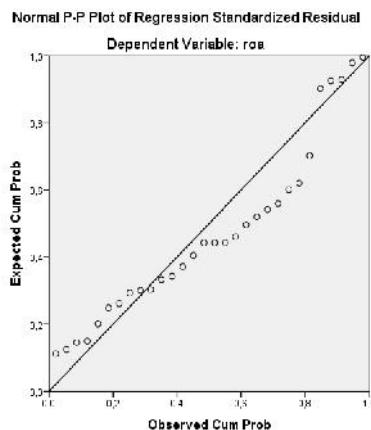
Gambar 3. Normal probability Plot
