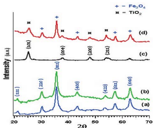
Figure 1. XRD pattern of (a). \text{Fe}_3\text{O}_4 , (b) \text{Fe}_3\text{O}_4/\text{SiO}_2 , (c). synthesized \text{TiO}_2 after calcinations at 500^\circ\text{C} , and (d). \text{Fe}_3\text{O}_4/\text{SiO}_2/\text{TiO}_2 composite through mechanochemical.
