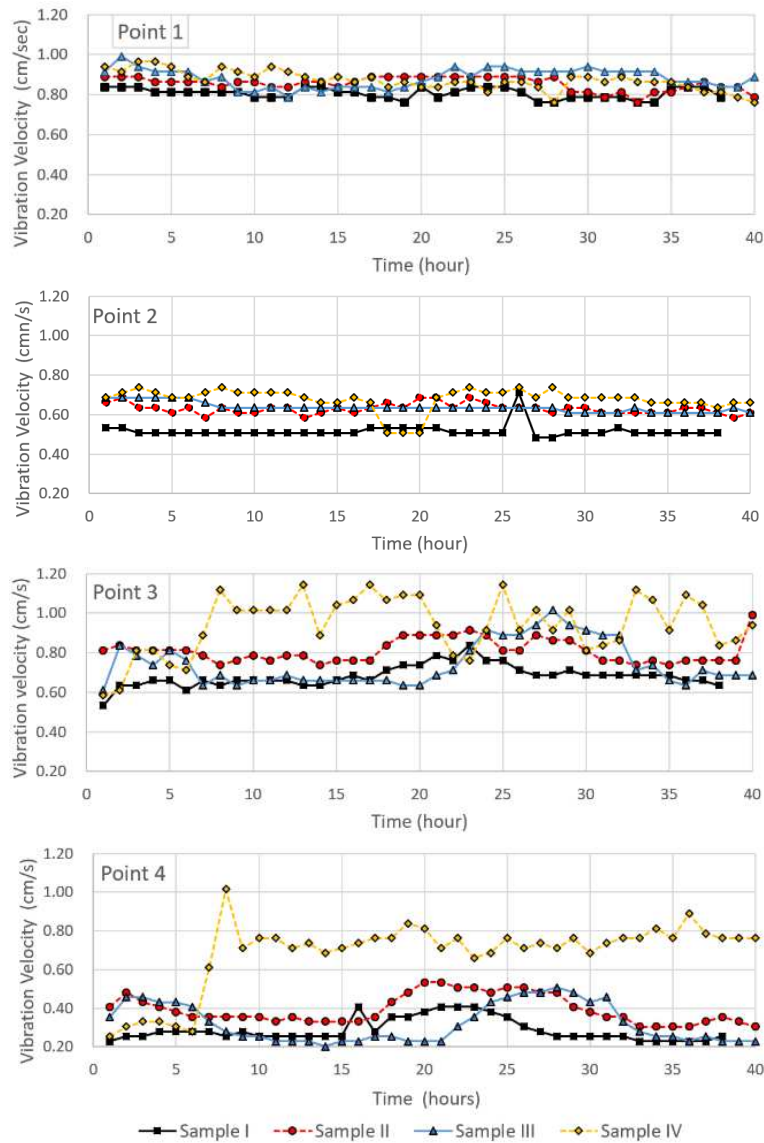
Figure 11. Vibration velocity profile
