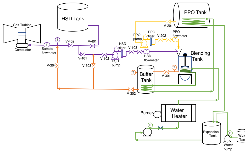
Figure 6. Sub-facilities of blending facility
