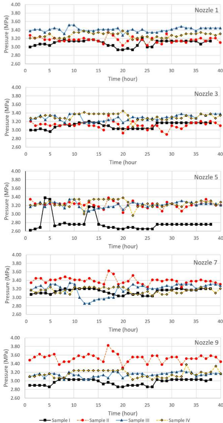
Figure 13. Nozzle pressure profile
