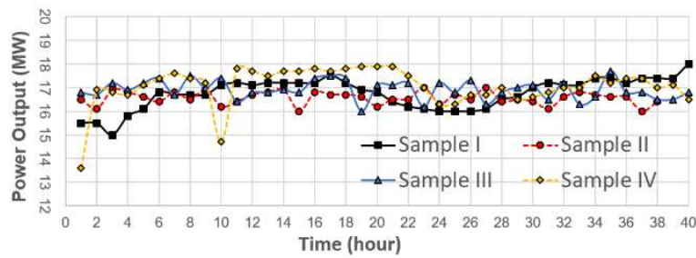
Figure 9. Power output
