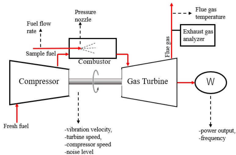
Figure 3. Flowchart of the experiment
