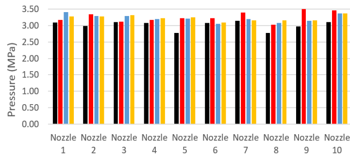
Figure 14. Average value of nozzle pressure
