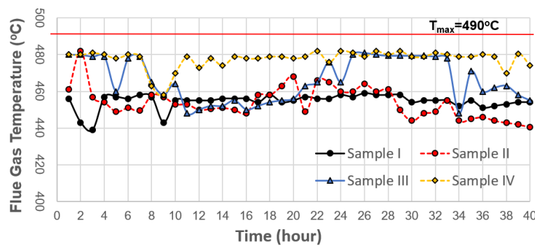
Figure 16. Profile of flue gas temperature
