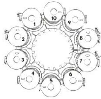
Figure 12. Combustor chambers [6]
