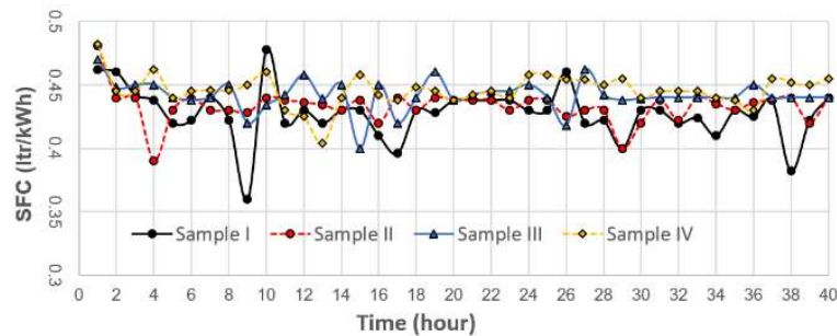
Figure 10. SFC profile
