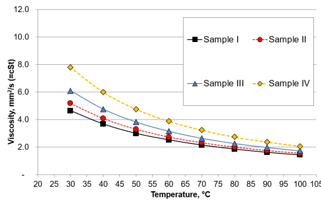
Figure 7. Effect of an increase in temperature on a sample viscosity
