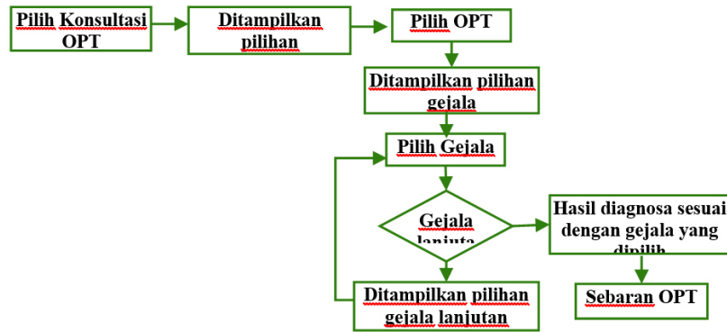
Gambar 5. Alur penalaran backward chaining
