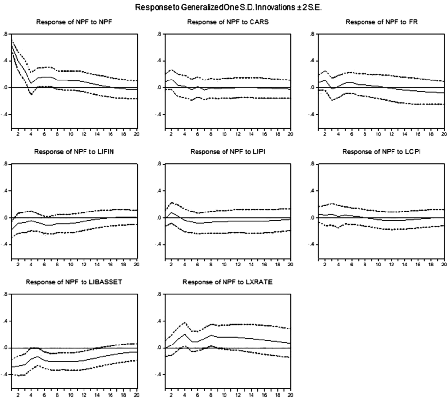
Figure 1. Impulse Response Function of NPF
