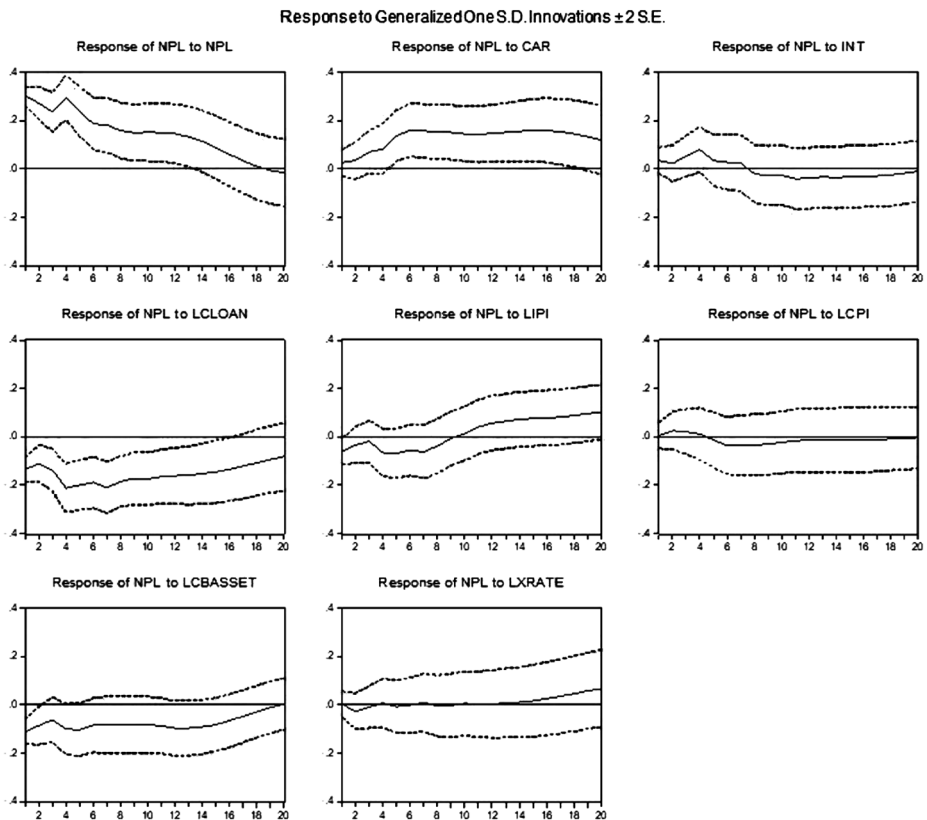
Figure 2. Impulse Response Function of NPL
