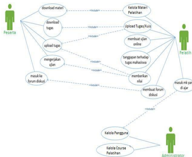
Gambar 2 Use Case Diagram pada E-learning Management System UPN “Veteran” Jakarta
