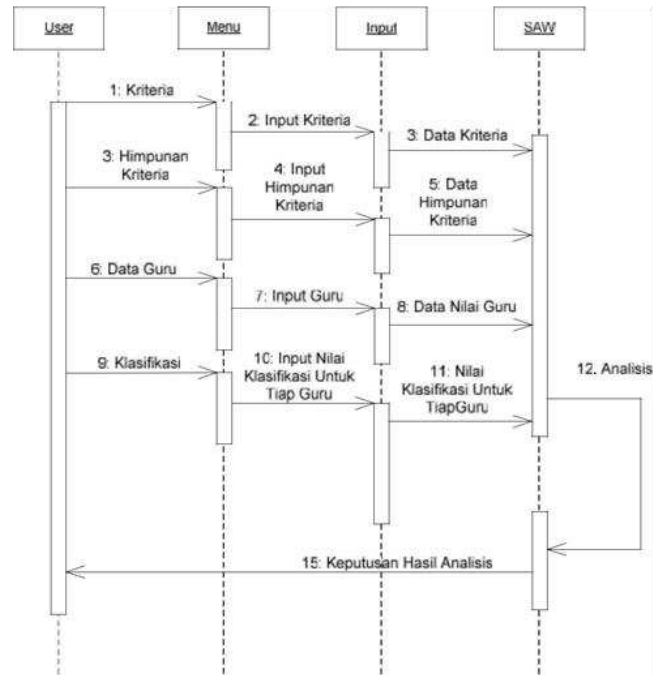
Gambar 6 Sequence Diagram Sistem
