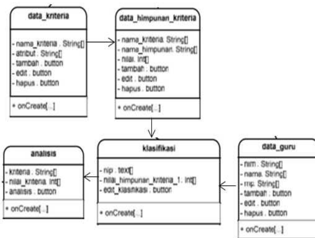
Gambar 3 Class Diagram Sistem
