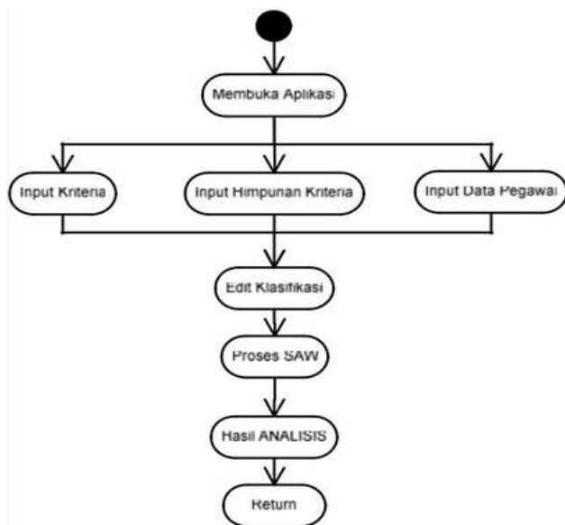
Gambar 5 Activity Diagram Sistem
