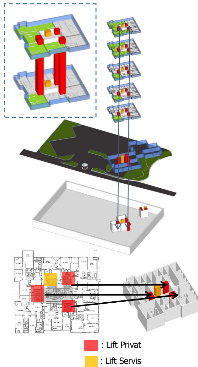
Gambar 11 Analisa Lift Privat Unit Tipikal Tower Avalon Apartemen Casa Grande Residence
