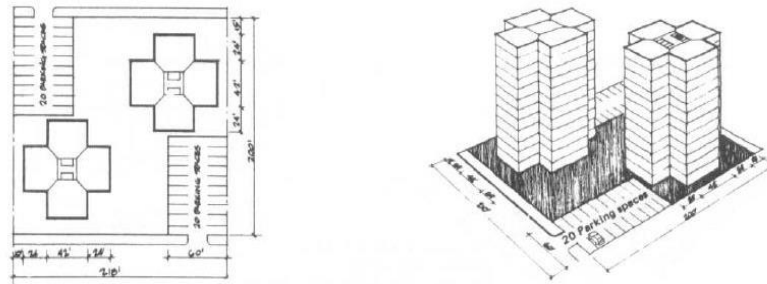
Fig. 12 Twin-tower apartments, density 94 units per acre.
