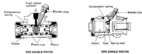
Gambar.8 Silinder Roda
