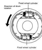
Gambar 3 Tipe Two Leading shoe
