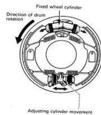
Gambar 6 Tipe Duo Servo
