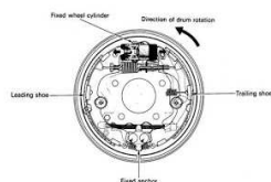
Gambar 2. Tipe leading trailing shoe
