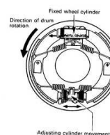
Gambar 5. Tipe Uni Servo
