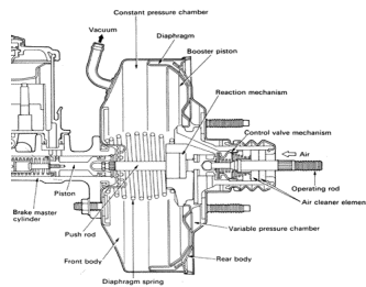
Gambar 11. booster rem
