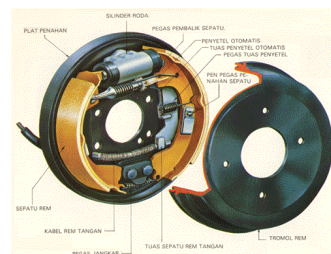
Gambar 10 Tromol Rem
