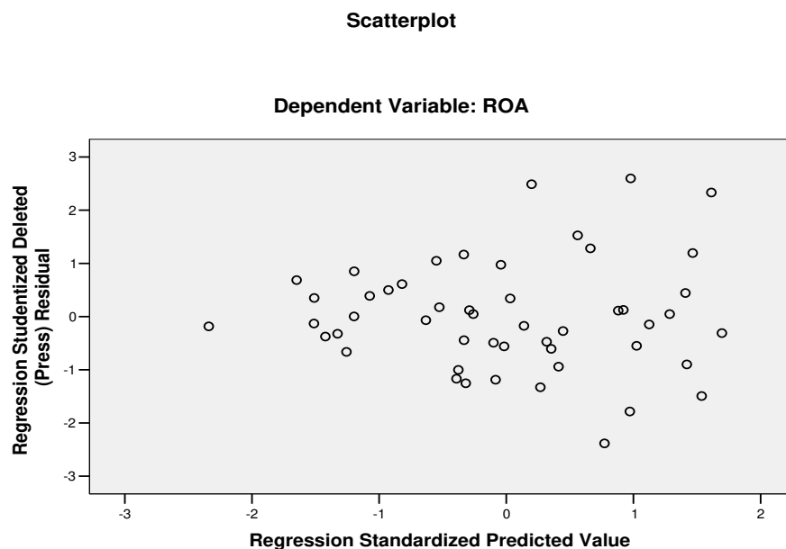
Gambar 2 Scatterplot
