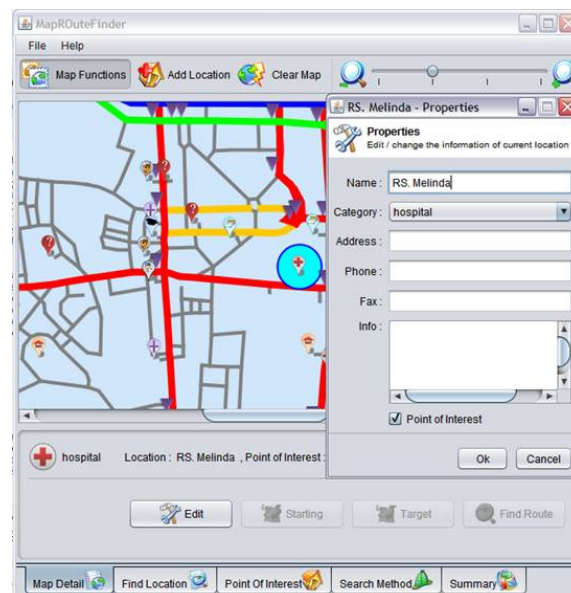
Gambar 8 Properties
