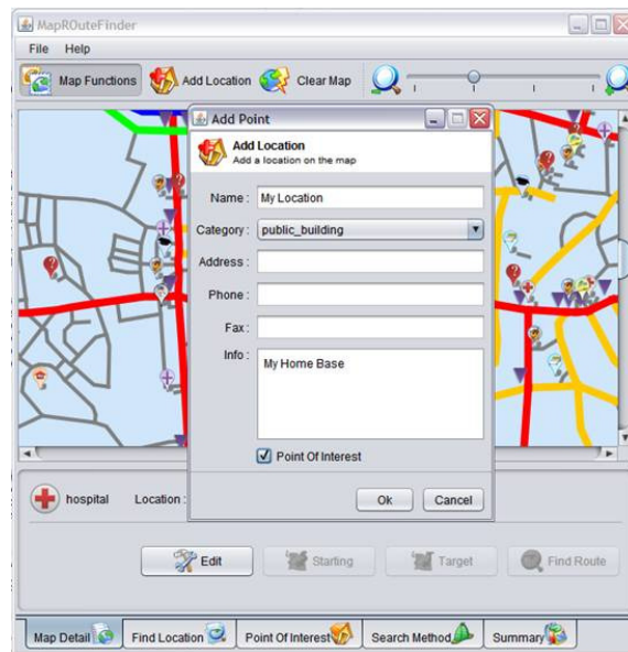
Gambar 9 Add Location
