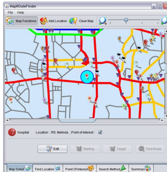
Gambar 7 Main Form
