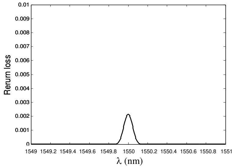
Figure 4. Return loss as a function of \Delta\lambda ; L=1\text{cm} , \kappa =5 \text{ cm}^{-1} , and \kappa_{ab}=0.5 \text{ cm}^{-1} .
