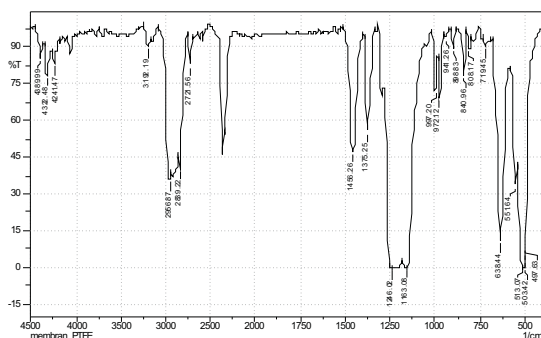
Figure 6. FTIR Spectra of PTFE Membrane
