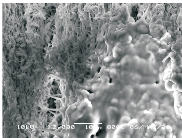
Figure 9. PTFE membrane impregnated with Didecillamine 4 \times 10^{-3} M using scanning electron microscope
