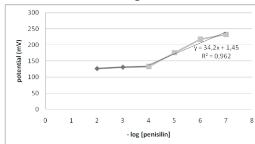
Figure 5. Nernst factor measurement from membrane impregnated with Didecillamine 2 \times 10^{-3} M and Penicilline 10^{-4} M with internal solution KCl 0,1 M and Penicilline 10^{-4} M in pH 8 Buffer Phosphate
