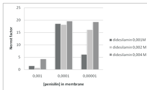
Figure 4. Nernst factor in membrane impregnated with Didecillamine and Penicilline (Internal Solution KCl 0,1 M and Penicilline 10^{-4} M)
