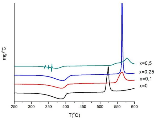
Gambar 16 Kurva DTG paduan Mg_{2-x}Al_xNi serbuk heat treatment 385^{\circ}C
