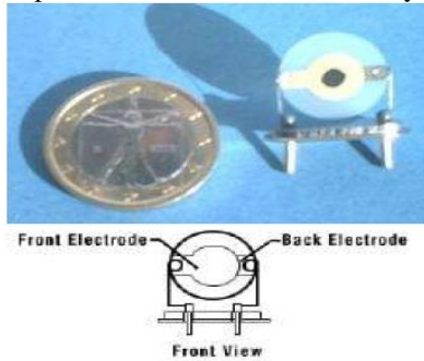
Gambar 1. Sensor QCM [3]
