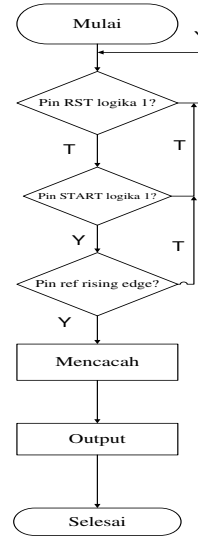
Gambar 6. Diagram alir blok counter
