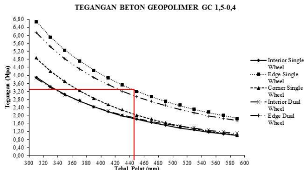
Gambar 8-Tebal Slab Minimum Beton Geopolimer GC-1,5-0,4
