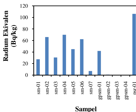
Gambar 4. Radium ekuivalen sampel semen (sm), gypsum (gpsm) dan pasir (psr)
