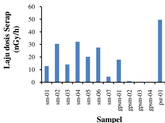
Gambar 8. Laju dosis serap sampel semen (sm), gypsum (gpsm) dan pasir (psr)
