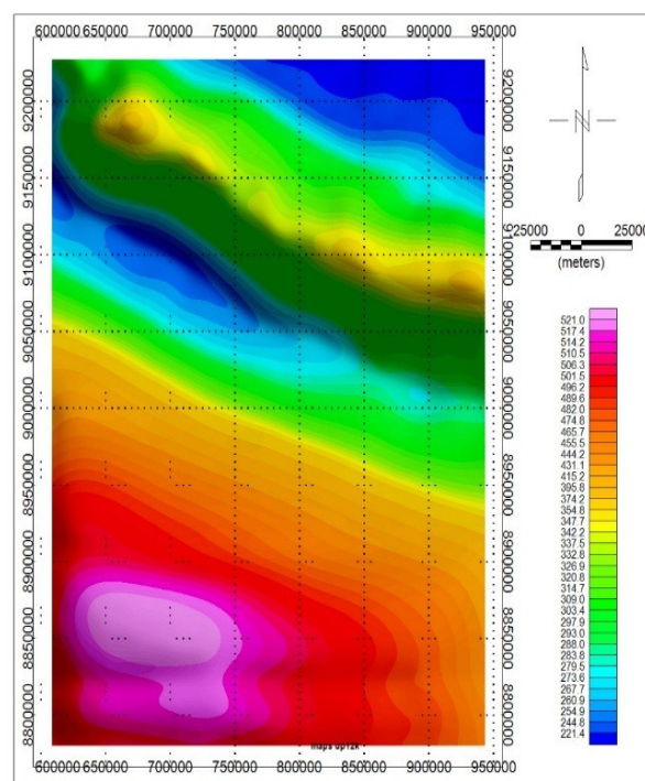
Gambar 3 Kontur anomali regional
