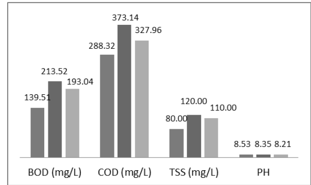
Gambar 3. Karakteristik limbah grey water
