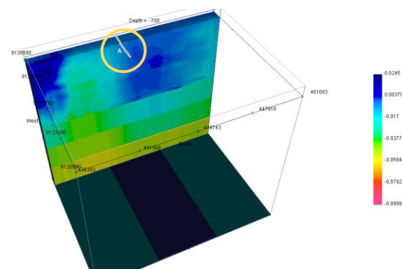
Gambar 4.7 Model 3D data anomali medan magnet
