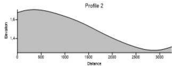
Gambar 4.5 Profil Second Vertical Derivative (SVD)
