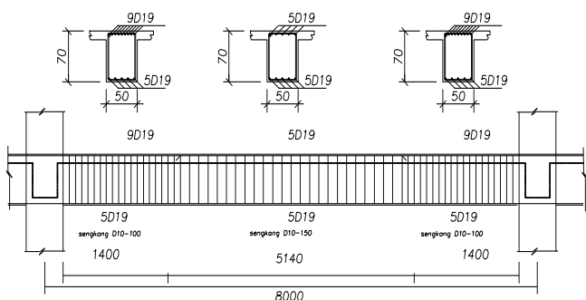
Gambar 4. Balok B1LT1
