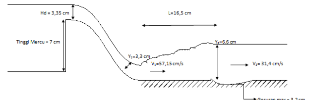
Gambar 7. Sketsa gerusan di hilir bendung model 1 debit 1,782 \times 10^{-3} \text{ m}^3/\text{det}
