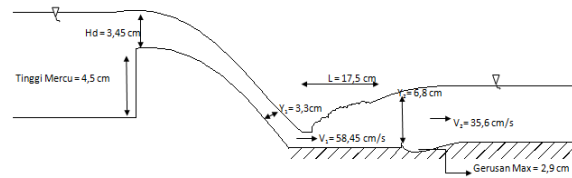
Gambar 15. Sketsa gerusan di hilir bendung model 1 debit 2,097 \times 10^{-3} \text{ m}^3/\text{det}
