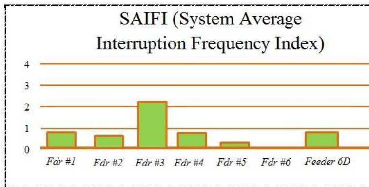
Gambar 4.4 Diagram Batang Nilai Indeks SAIFI Feeder GI 6D
