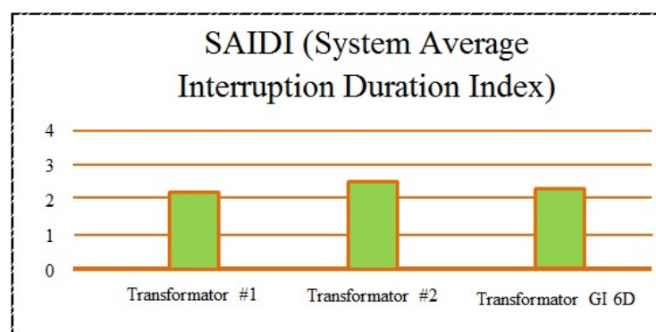
Gambar 4.1 Diagram Batang Nilai Indeks SAIDI Transformator GI 6D
