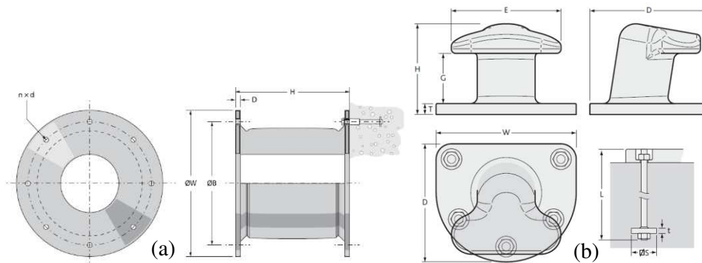
Gambar 9 (a) Cell Fender (b) T-head bollard
