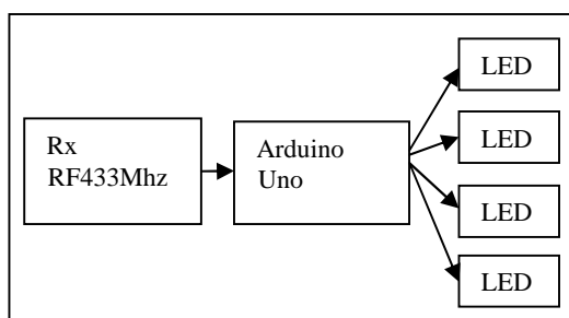
Gambar 5.2 Desain Rangkaian Receiver
