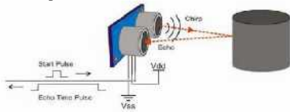
Gambar 4.3 Sensor Ultrasonik
