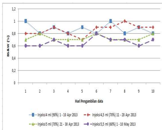
Gambar 2. Percobaan lapangan tentang hubungan injeksi demulsifier 4,0 ml (90%), 4,5 ml (70%), 5,0 ml (70%) dan 5,5 ml (60%) terhadap BS&W
