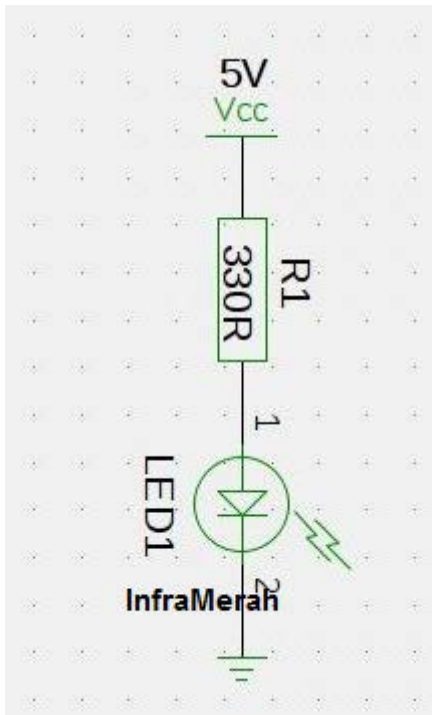
Gambar 3.3 Rangkaian sensor Infrared
