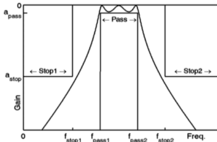
Gambar 6. Respon Filter BPF (YYePG, 2004)
