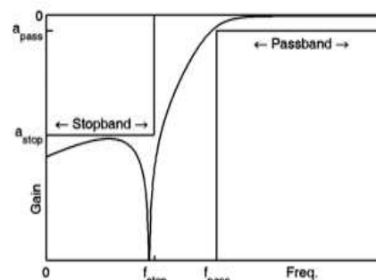
Gambar 5. Respon Filter HPF (YYePG, 2004)
