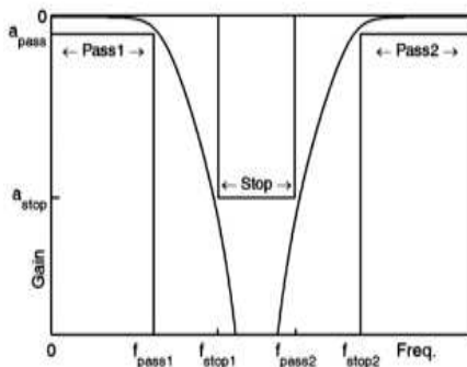
Gambar 7. Respon Filter BRF (YYePG, 2004)
