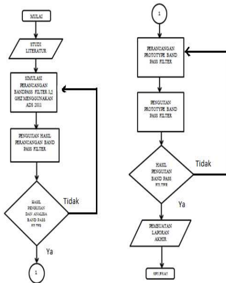
Gambar 10. Diagram Alir Desain Band Pass Filter
