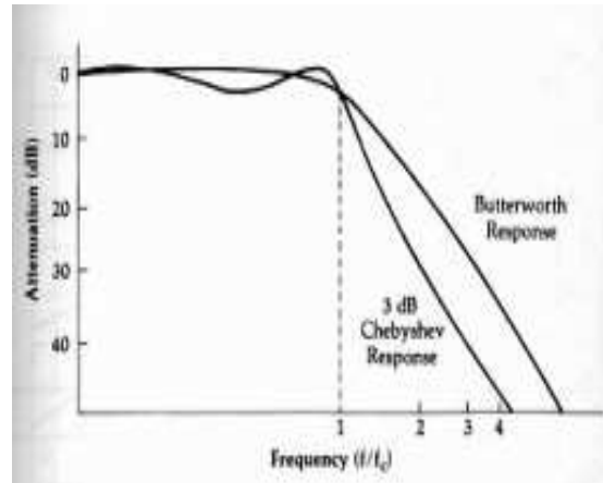
Gambar 8. Respon Frekuensi Chebyshev Filter dan Butterworth Filter (YYePG, 2004)
