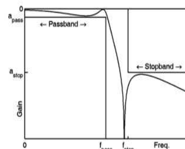
Gambar 4. Respon Filter LPF (YYePG, 2004)
