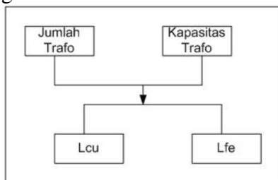
Gambar 8. Bagan Perhitungan Rugi-rugi Trafo Distribusi
