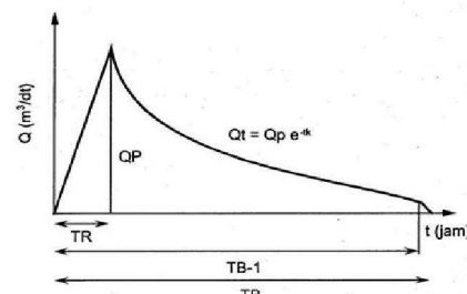
Gambar 4. HSS Gama I
