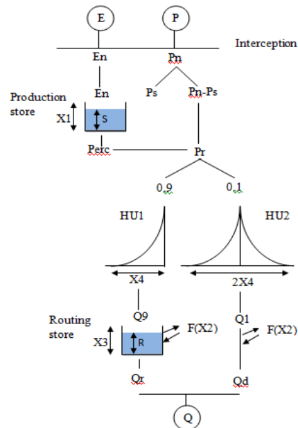
Gambar 2. Diagram model rainfall-runoff GR4J (Perrin, 2003)
