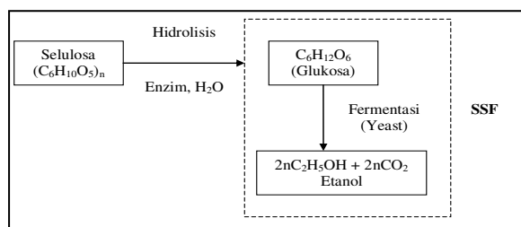
Gambar 1.1 Skema reaksi dalam proses Simultaneous Sacharification and Fermentation (SSF)
